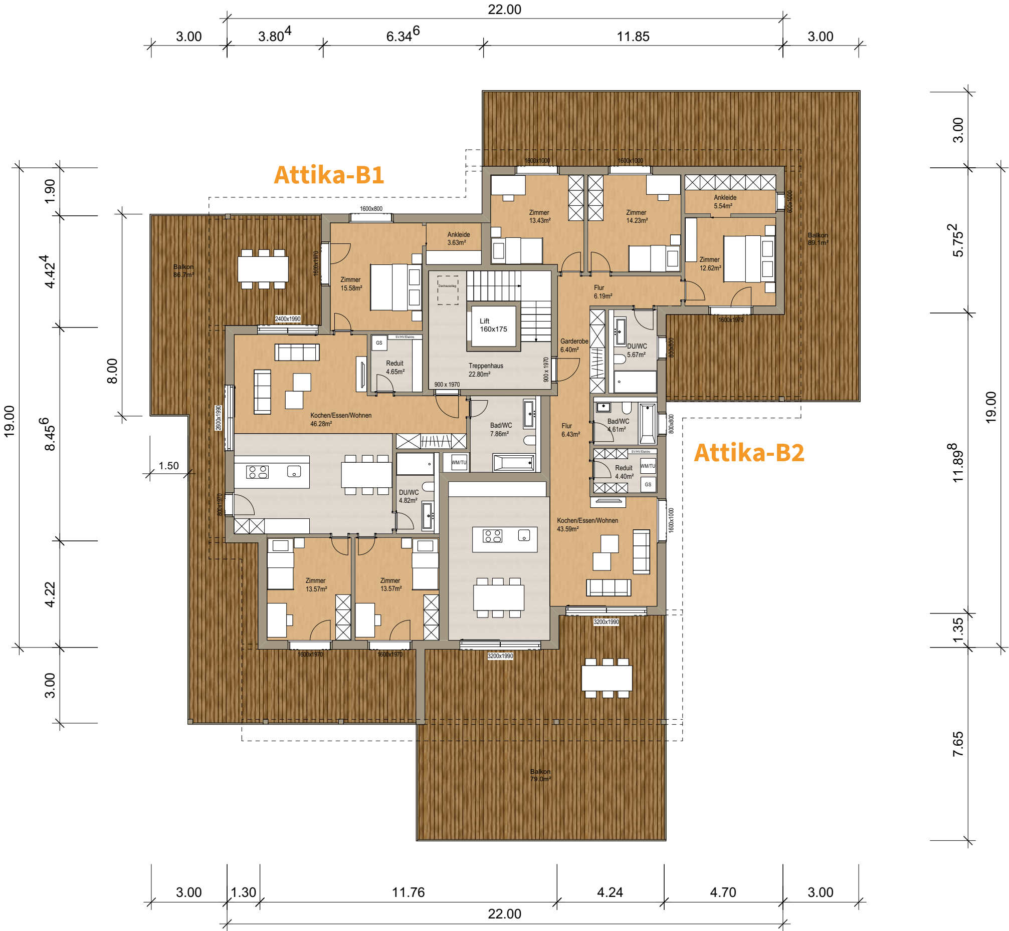
Grundriss Attika MST:1:150
